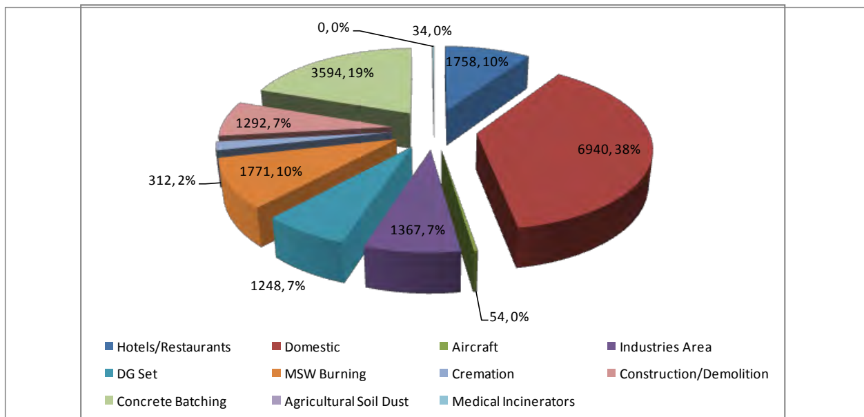
Figure 3.50: PM 2.5 Emission Load for area sources (kg/day, %)
