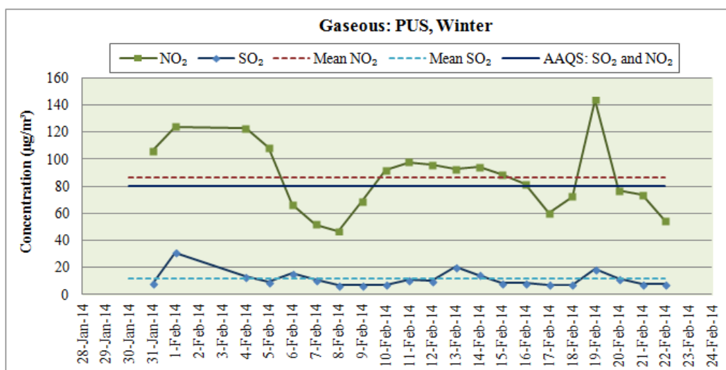
Figure 2.68: SO 2 and NO 2 Concentrations at PUS for Winter Season
