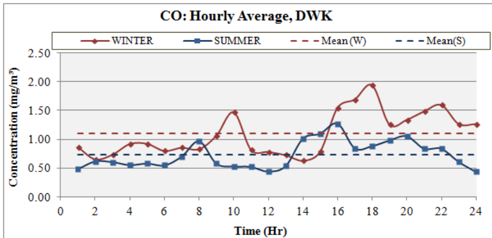
Figure 2.33: Hourly average concentration of CO at DWK for winter and summer seasons
