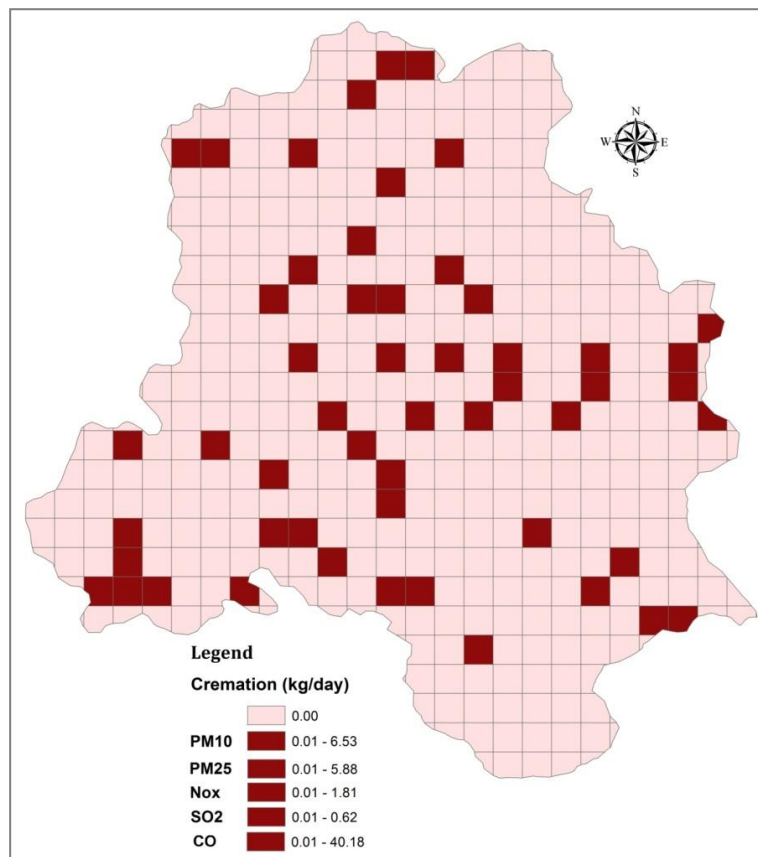
Figure 3.39: Spatial Distribution of PM 10 , PM 2.5 , NO x , SO 2 , CO Emissions from Cremation Sites
