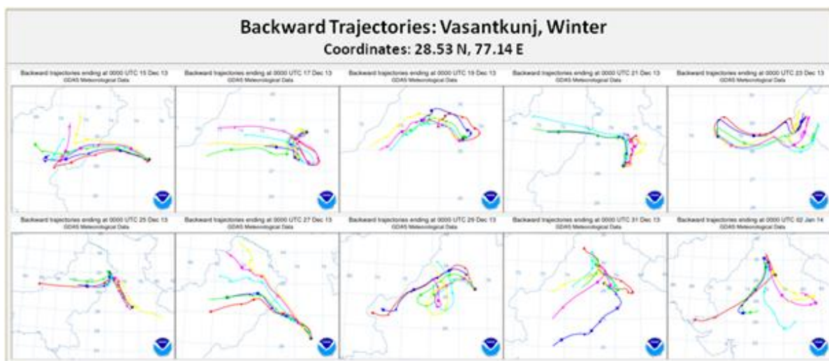
Figure 4.21: Backward trajectories at VKJ for Winter Season
