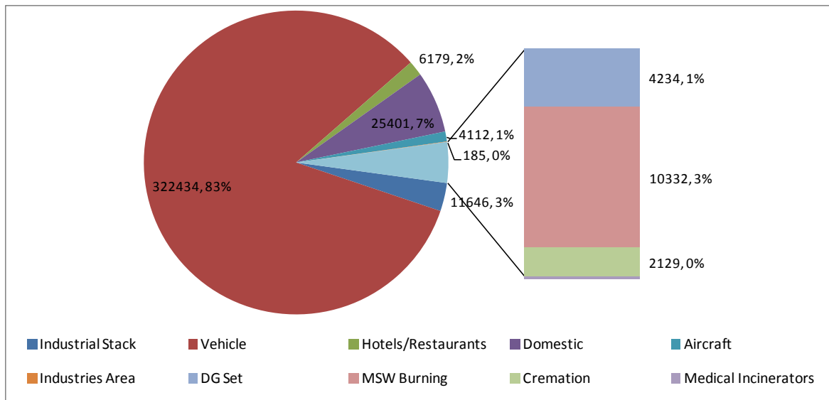
Figure 3.83: CO Emission Load Contribution of Different Sources in the City Of Delhi
